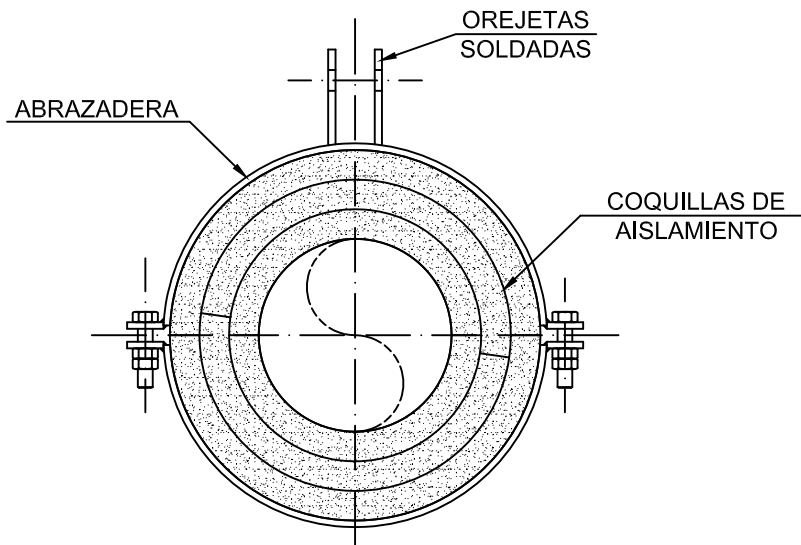
VISTA X-X
